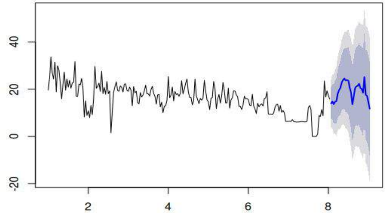
Forecasts from HoltWinters
